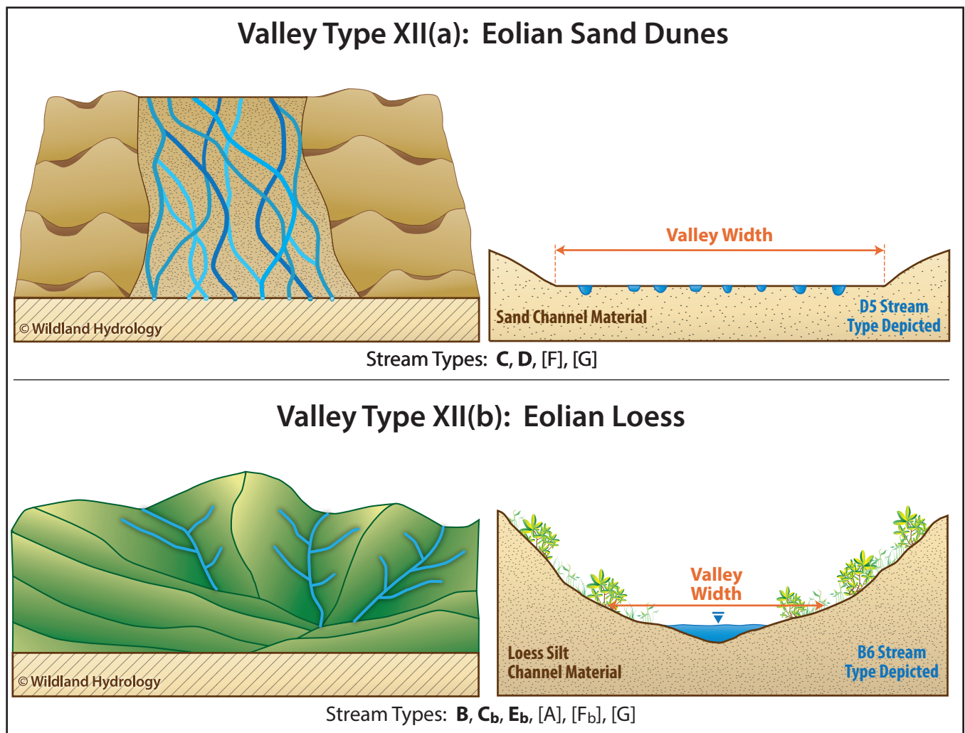
Figure B-30. Valley Type XII(a), eolian sand dunes, and Valley Type XII(b), eolian loess.
