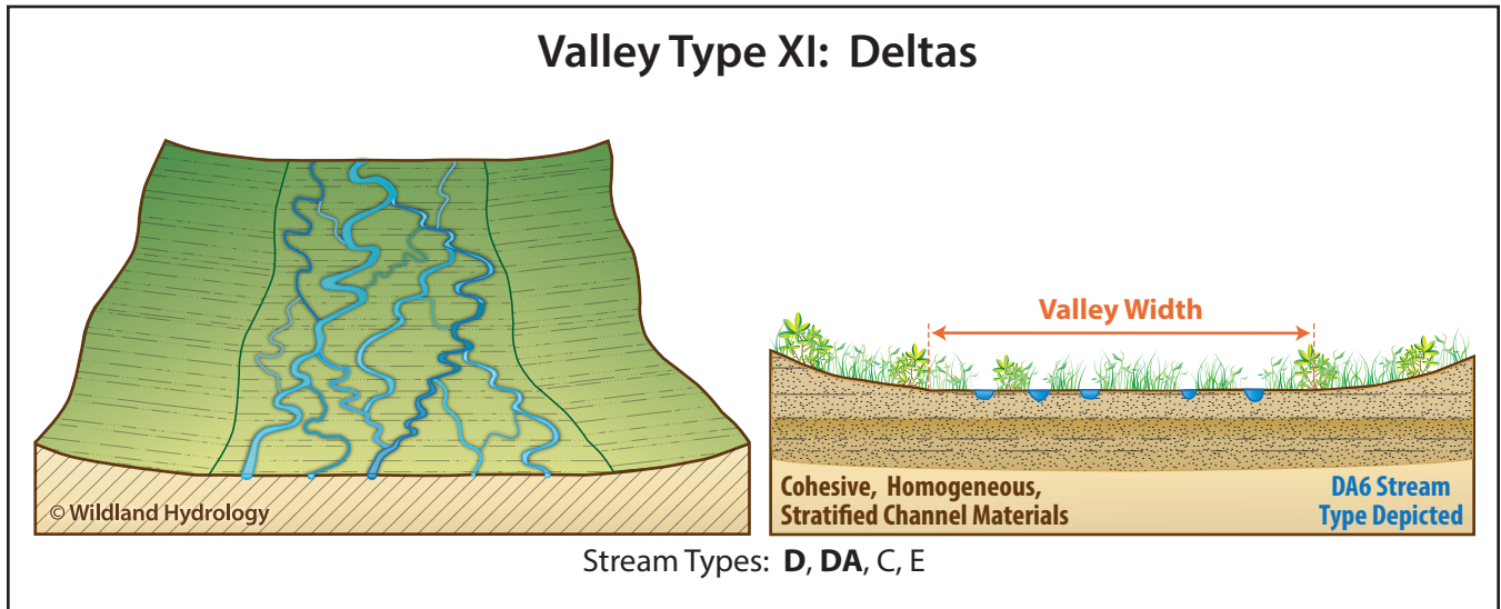
Figure B-28. Valley Type XI, Deltas.
